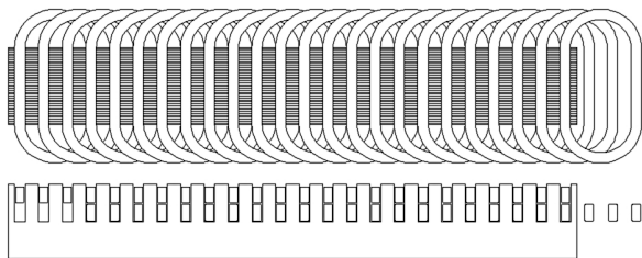
Fig. 1. 8 pole double layer winding layout
