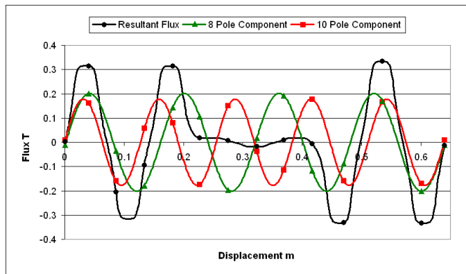
Fig. 3b. 9 coil stator air gap flux and harmonic components at 120^\circ
