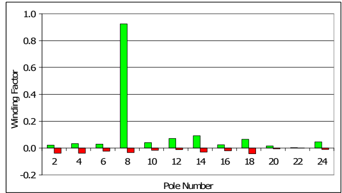
Fig 6. Winding factors of the wound rotor
