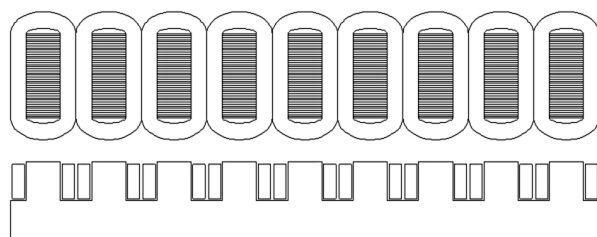
Fig. 2. 8 pole modular winding layout
