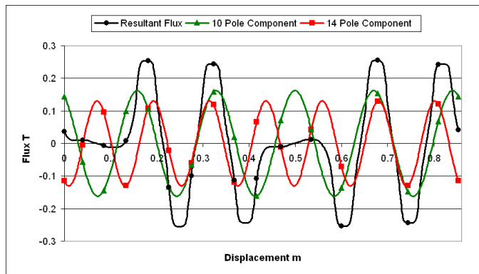
Fig. 4a. 12 coil stator air gap flux and harmonic components at 0^\circ
