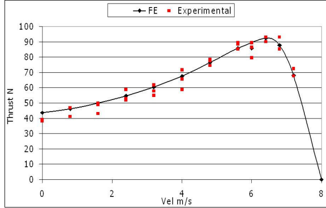
Fig. 7. Wound rotor experimental and FE results
