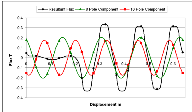
Fig. 3a. 9 coil stator air gap flux and harmonic components at 0^\circ
