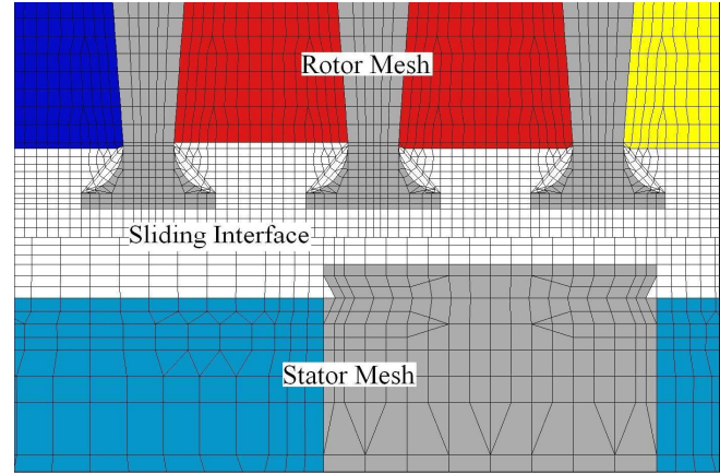
Fig. 8. A finite element mesh
