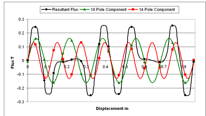
Fig. 4b. 12 coil stator air gap flux and harmonic components at 120^\circ
