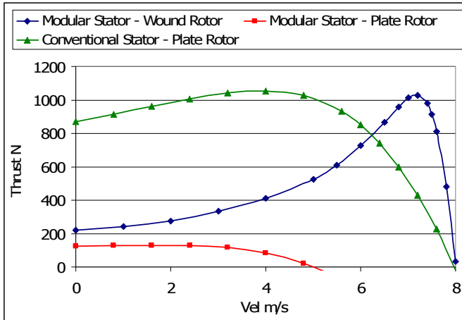
Fig. 5. Thrust speed curves for modular stator with both plate and wound rotors, and conventional stator with plate rotor
